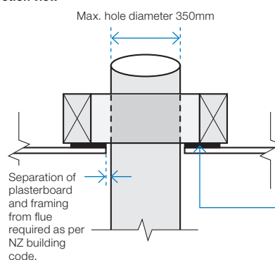
FIGURE 25: SERVICES, PENETRATIONS AND RANGE HOOD OPENINGS
