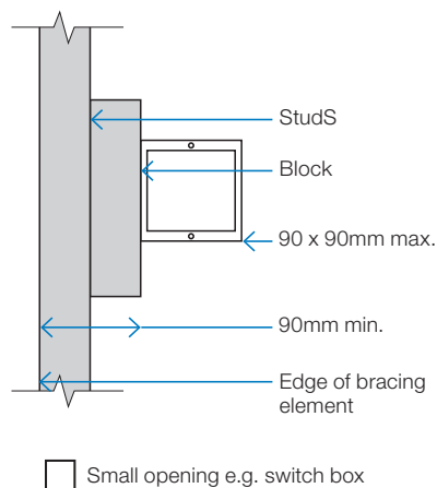
FIGURE 10: SMALL OPENINGS IN BRACING ELEMENTS
