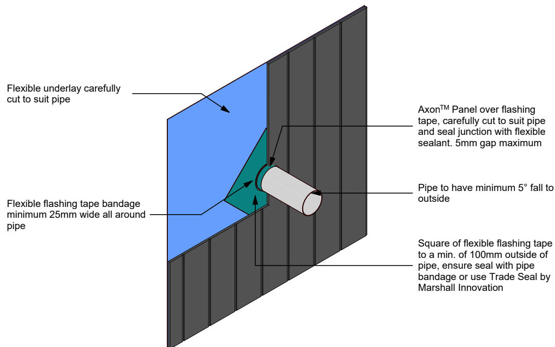
Figure 27: Cavity pipe penetration
