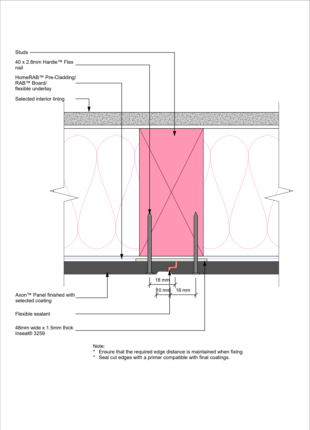
Figure 4: Axon™ Panel vertical shiplap joint — Hardie™ Flex nail
