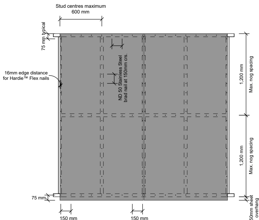
Figure 28: Direct fixed typical panel brad nail fixing setout
