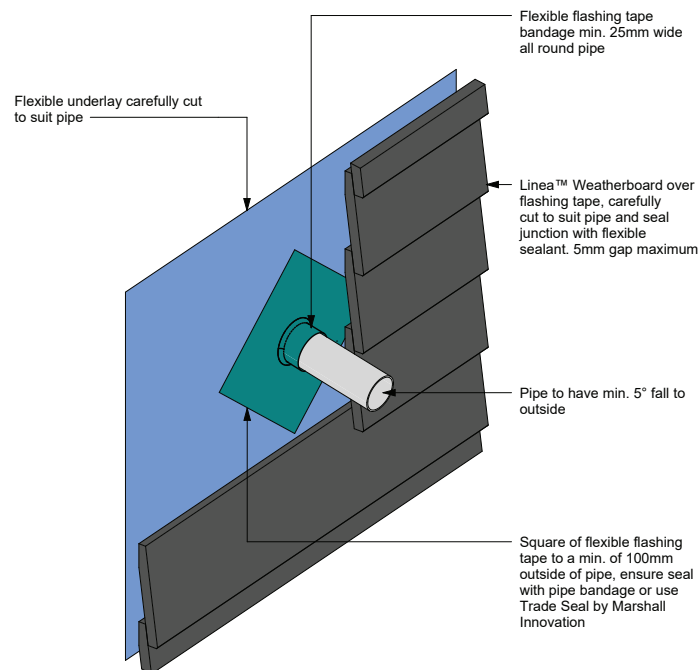
Figure 19: Pipe penetration
