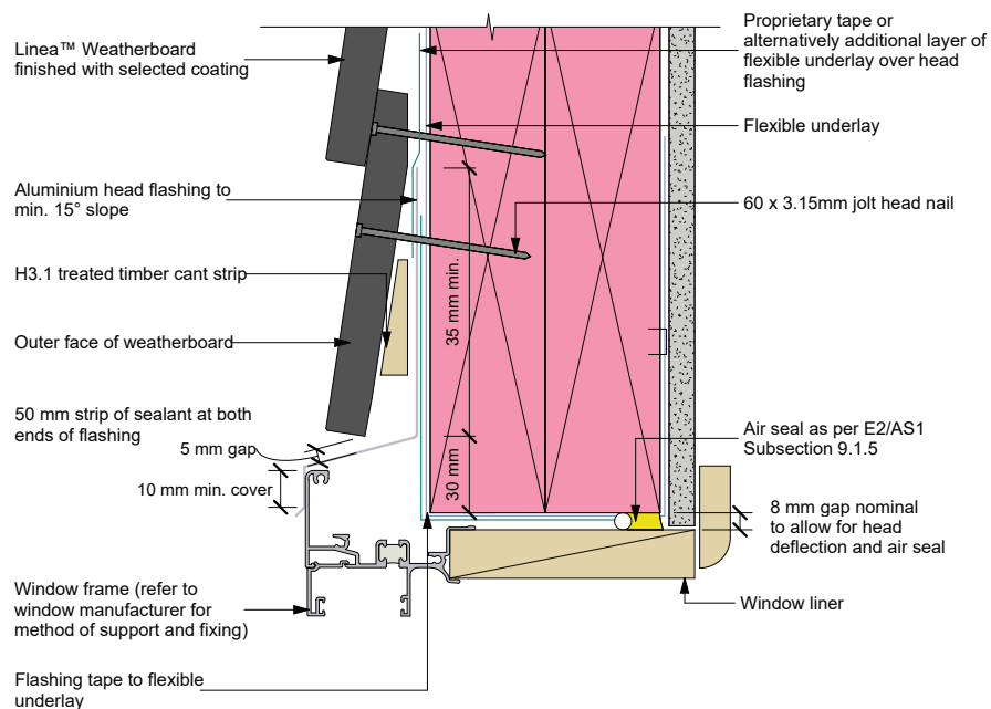
Figure 13: Window head
