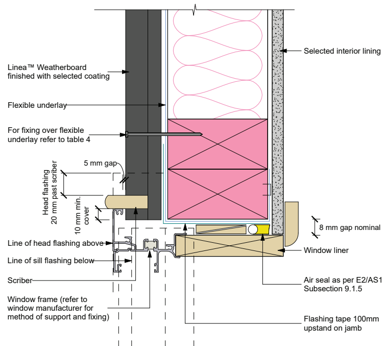
Figure 14: Window jamb
