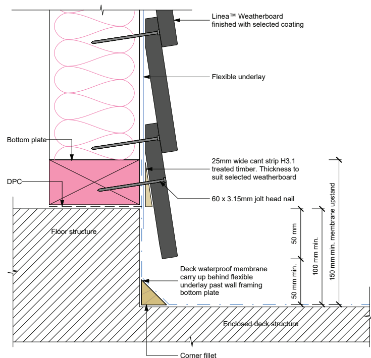
Figure 3: Enclosed deck
