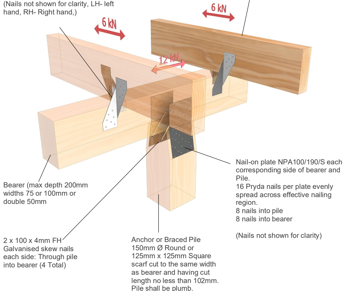
DETAIL 1: 12 kN HORIZONTAL CAPACITY FIXING OF BEARER TO CANTILEVER PILE AND 2 X 6 kN JOIST TO BEARER IN ACCORDANCE WITH NZS 3604:2011 CLAUSES 6.8.6.1
